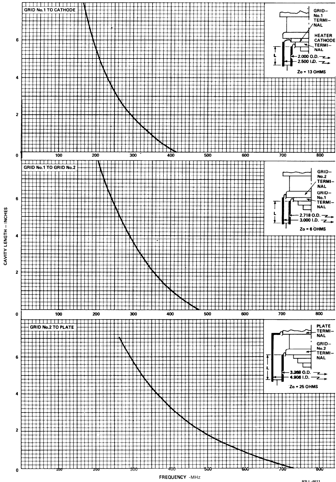
Figure 9 -Tuning Characteristics
