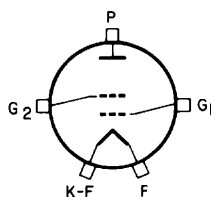
Figure 7 - Terminal Diagram
