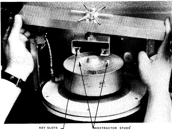
Figure 10 - Tube Puller J15449 for Use with BURLE Tube Type 8806
