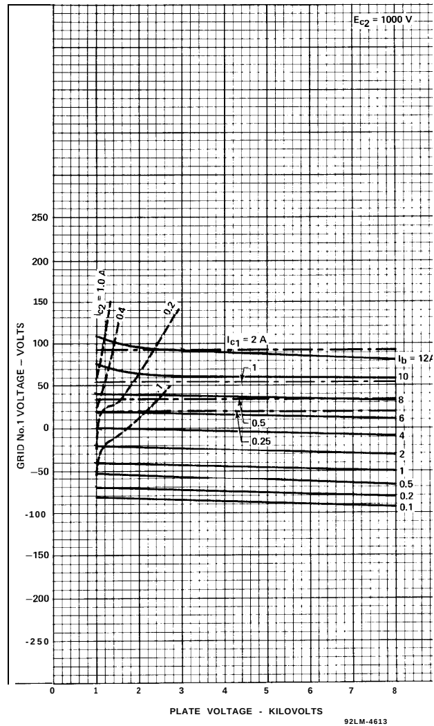
Figure 2 - Typical Constant Current Characteristics E_{C2} = 1000V
