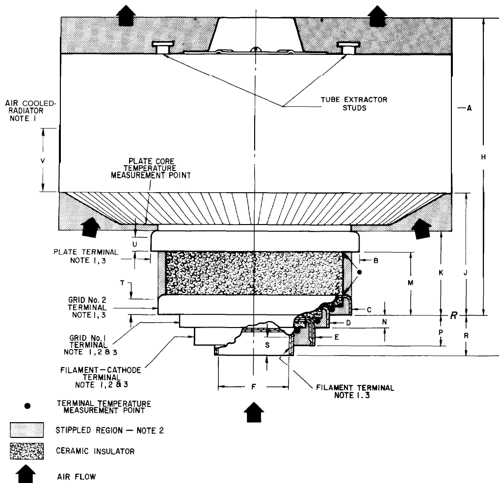
Figure 5 - Dimensional Outline
